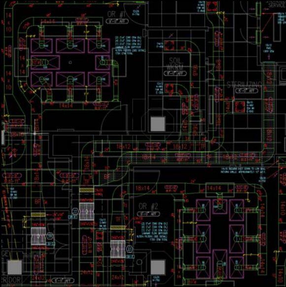
HVAC SHOP DRAWINGS
