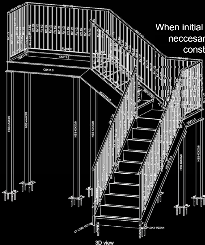
STEEL SHOP DRAWINGS
